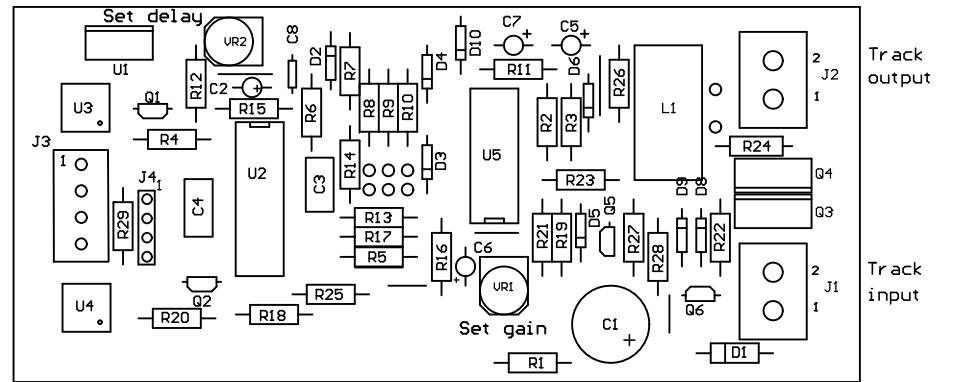
BDC1 Cutout & block detector Rev F
