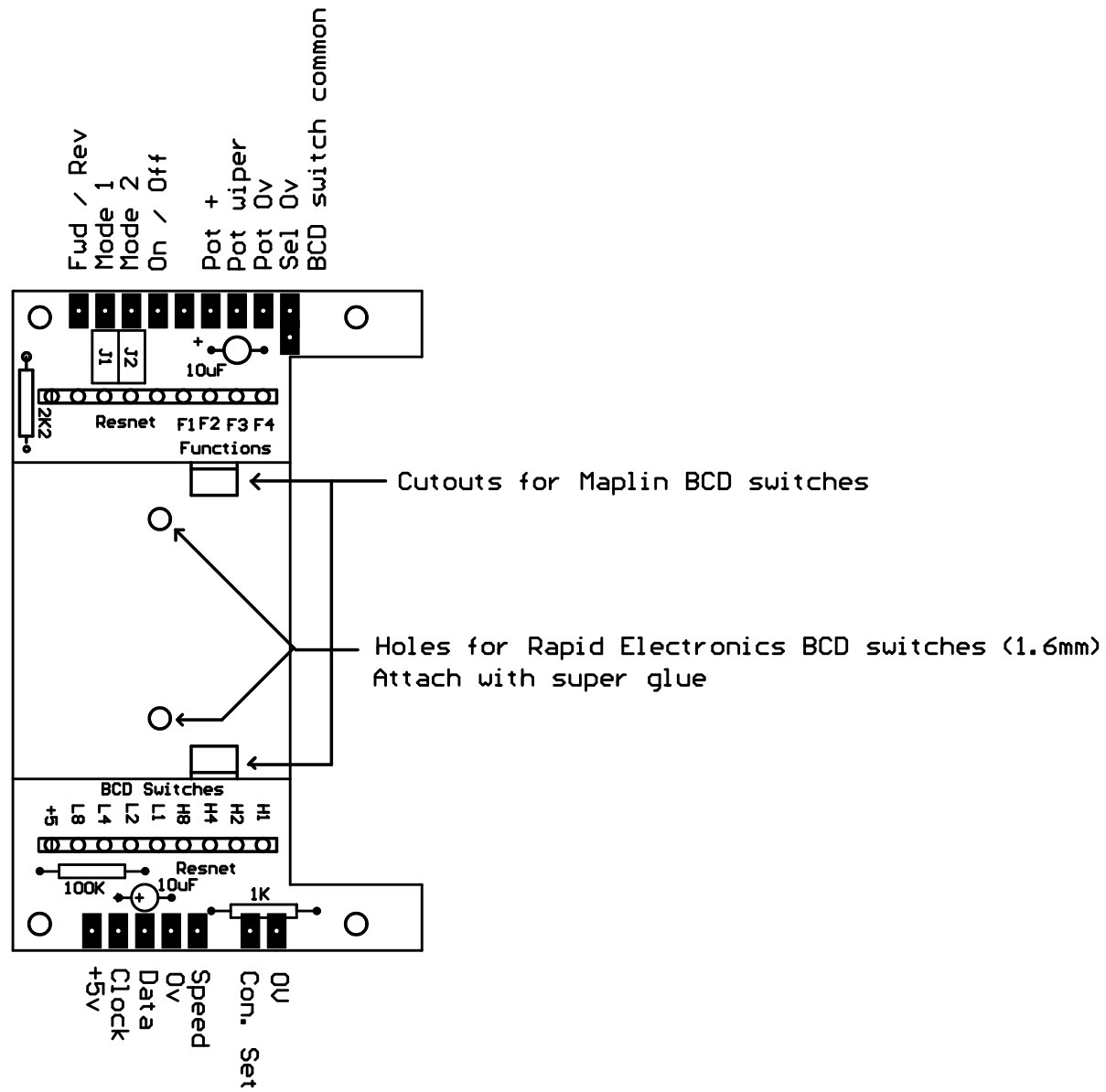
View from BCD switch side
