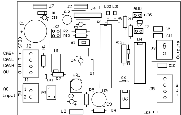
CANCMD CBUS Programmer and command station / booster module
