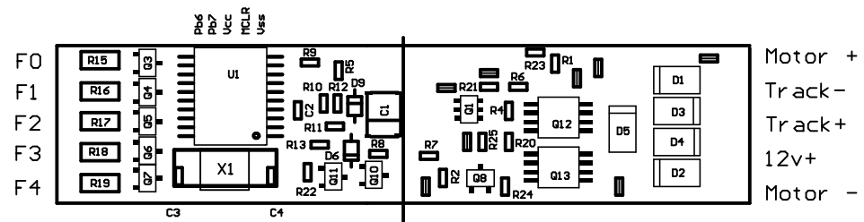
MERG Decod 11 Rev A 1/4/00
